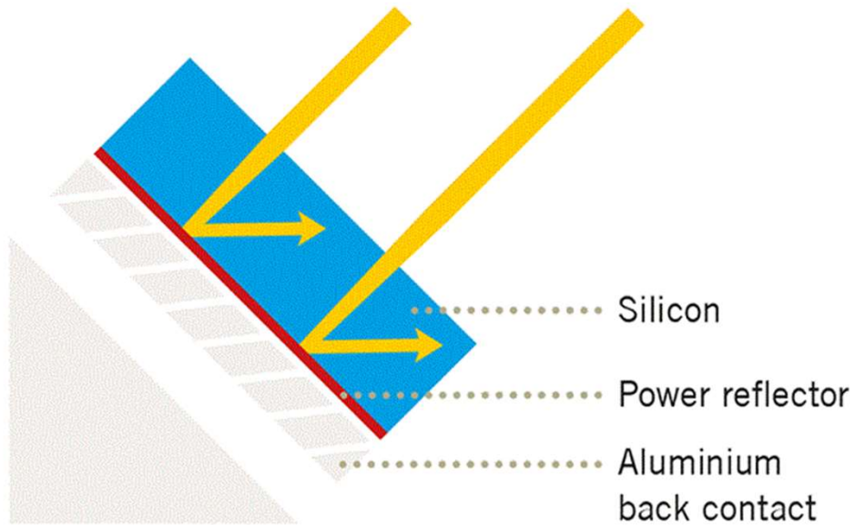
Q.ANTUM solar cell from Q CELLS
