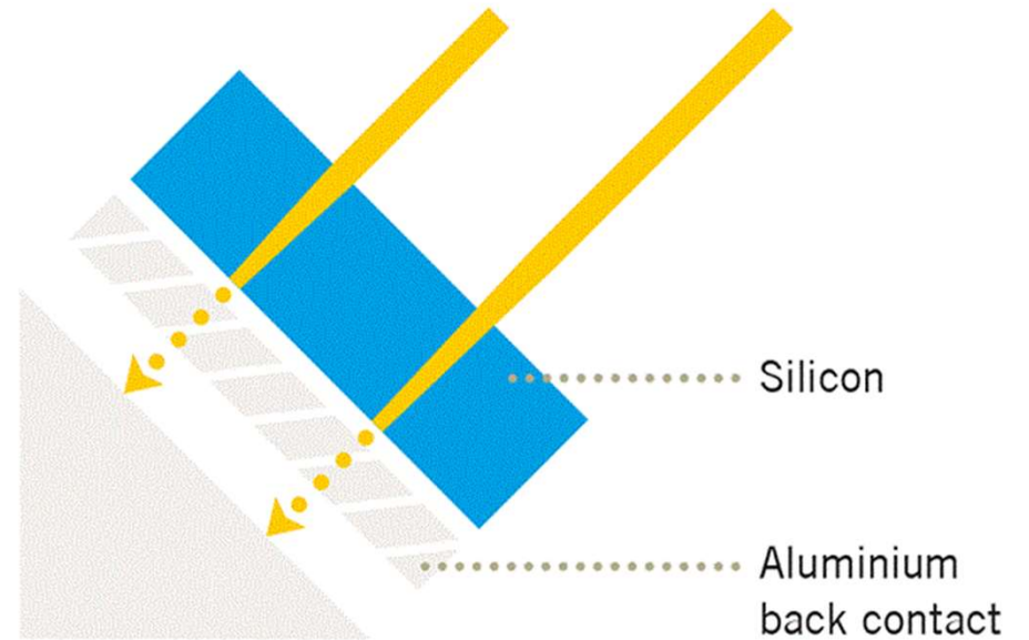
Polycrystalline standard solar cell
