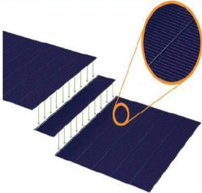
Tiled-cell panel Solar Cells
