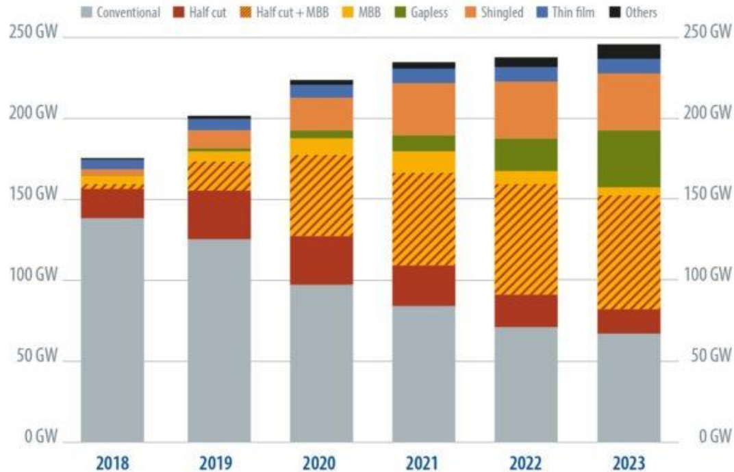
Module capacity forecast
